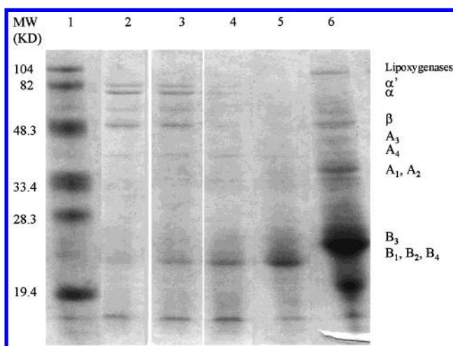
Figure 6. Urea-SDS-PAGE of protein permeate samples obtained from UF with RC-100 membrane at different recirculation speeds (RS): (lane 1) MW standards; (lane 2) 300 L/min RS; (lane 3) 250 L/min RS; (lane 4) 200 L/min RS; (lane 5) 150 L/min; (lane 6) 100 L/min RS. \alpha , \alpha' , and \beta are peptide bands of \beta -conglycinin. A and B are the respective acidic and basic peptides of glycinin. Thirty micrograms of protein was loaded per well.
